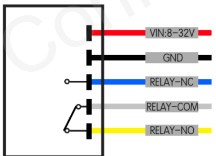
Enable relay
