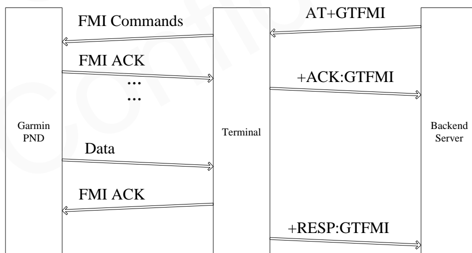
Figure 1: @Tracker for Garmin-FMI Protocol Message Flow
