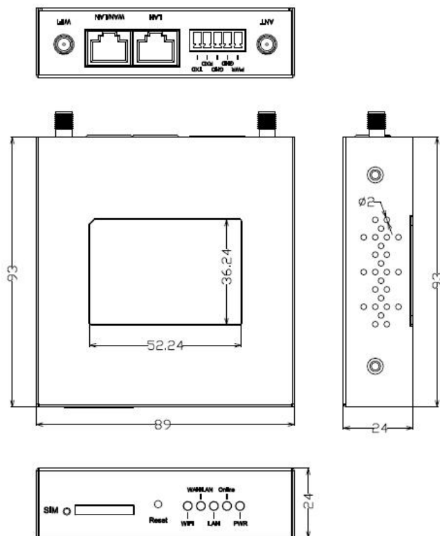
DIN Rail Style Router Dimension
