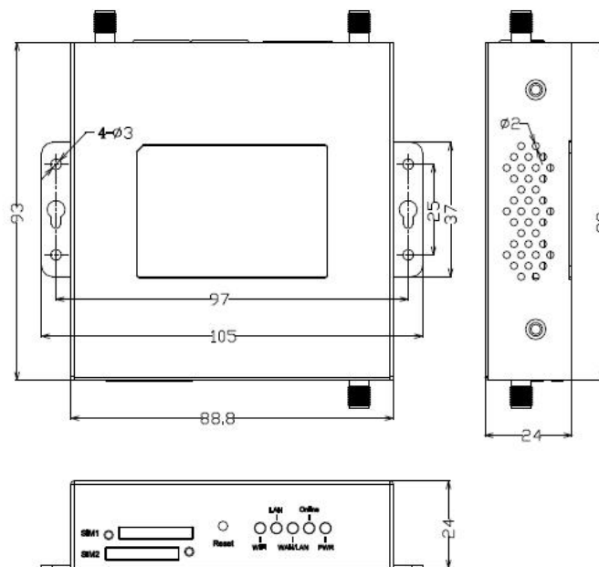
Wall Mount Style Router Dimension
